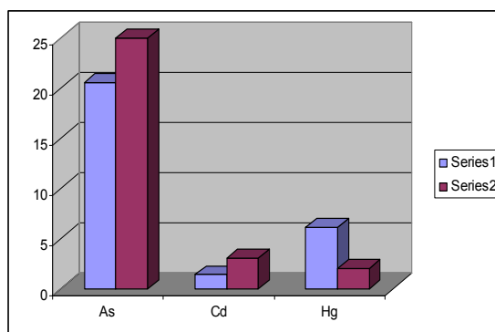
Graph 4. The contents of arsenic, cadmium and mercury, compared to MAC
