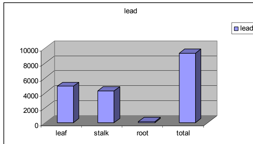
Graph 1. Disposition of the adopted lead in the plant phytoaccumulator
