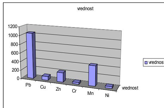
Graph 3. Heavy metals in the soil
