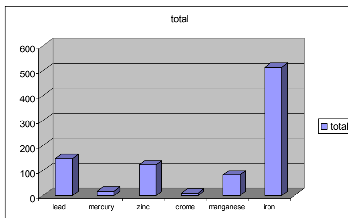
Graph 5. Heavy metals phytoaccumulated from the soil
