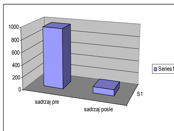
Graph 2. The lead content in the soil before and after application of the Phytoremediation
